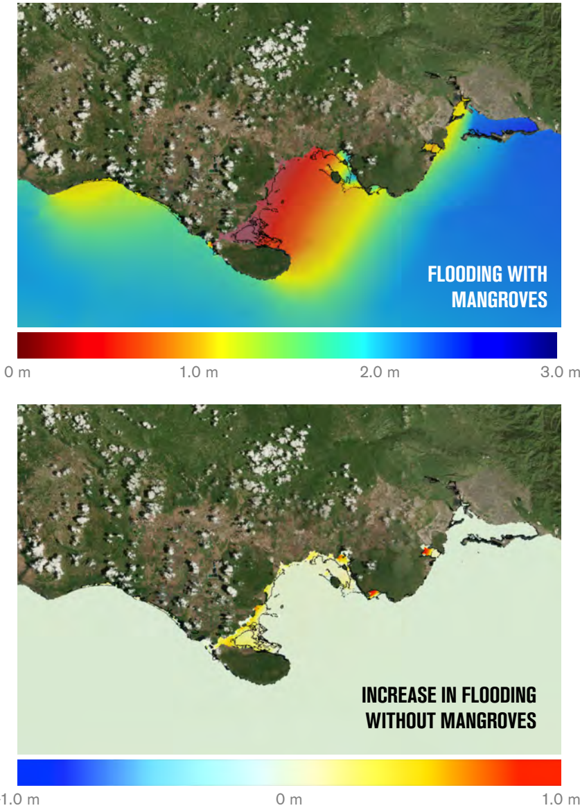
FIGURE 21 Storm surge along the southwestern Jamaica produced by hurricane Dean in August 2007 for the mangrove scenario (upper panel) and differences of removing mangroves from the model setup (bottom panel).
